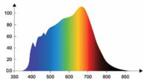
Resemble solar spectra
